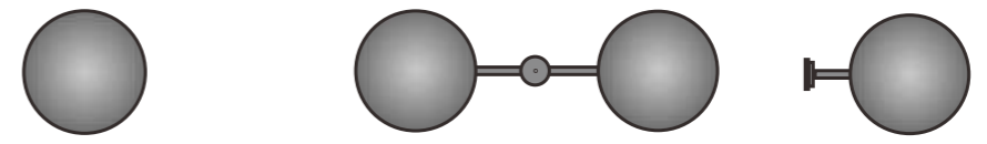
Single (1) Die cast aluminum fitter base secured to pole with two stainless steel, Allen head set screws. Double (2) Double luminaire mounting arm secured to pole with four stainless steel, Allen head set screws. Wall (W) Double wall mount arm secured to wall with
